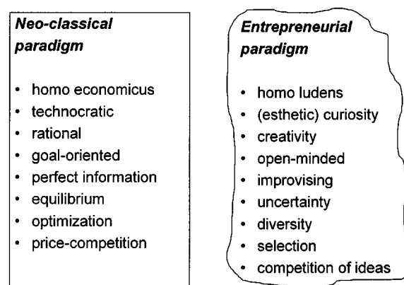
Figure 2. Two paradigms.
